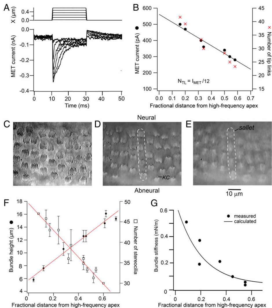
Fig. 3. MET in salletal hair cells. (A) MET currents in response to step deflections of the hair bundle (Upper) at -84 mV holding potential. (B) Tonotopic variation in peak MET current amplitude (black circles) for seven hair cells, and number of tip links (red crosses) derived by assuming each tip link is connected to two 6-pA MET channels. (C–E) Endolymphatic surface of the abneural aspect of the papilla in the salletal region ( d = 0.5 ) focused at three different heights: (C) base of bundles, used to count the number of stereocilia; (D) top of the bundles, showing the kinocilium (KC), used to determine bundle polarity. Note that in each row of bundles under a given sallet, there is a reversal in bundle polarity about halfway across the papilla. (E) The sallets, used to determine the number of hair bundles per sallet; dotted white line emphasizes sallet location. (F) Plots of stereociliary number determined from live sections as in C and bundle height determined from tallest stereocilia when the cell was pushed on its side. Each measurement, \pm SD, was made on four hair bundles, including oppositely oriented polarities, at each location in two preparations. (G) Tonotopic variation in hair bundle stiffness versus cell location. Smooth curve was calculated (Results) from bundle height and number of stereocilia assuming the rotational stiffness of a stereocilium as 4.6 \times 10^{-16} N.m/rad. Filled circles are discrete measurements on single hair bundles, as described in Methods (25).
