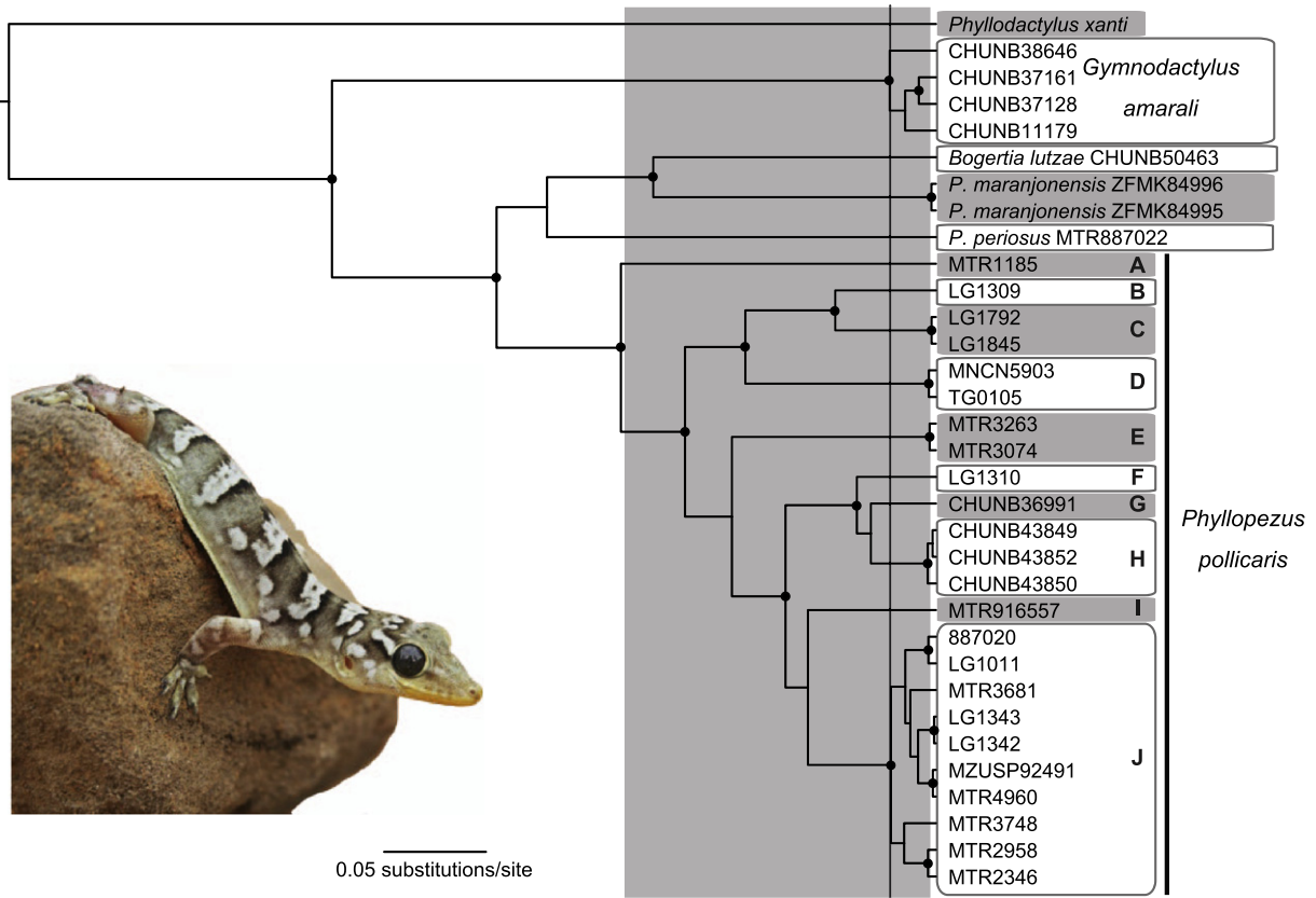
Fig. 4. Ultrametric phylogeny of unique 16S haplotypes. The vertical line represents the cutoff for species-level clusters identified by the GMYC analysis. Taxon names/IDs of species-level clusters are enclosed by boxes. The large gray box shows the confidence interval of species-level clusters (6–25 clades). Circles indicate nodes with posterior probabilities >0.95. Photo of Phyllopezus periosus by MTR.
