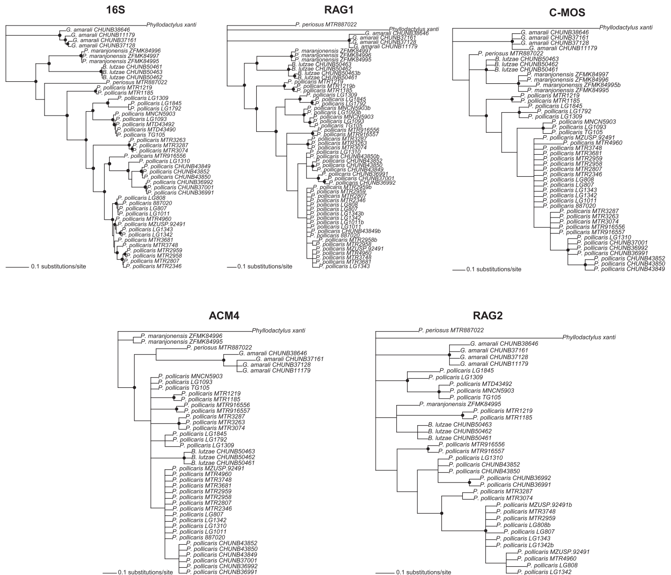
Fig. 3. Bayesian phylogenies for each locus. Circles at nodes indicate clades with posterior probabilities >0.95 . Taxon names appended with a "b" represent the alternative phased allele for heterozygous individuals.
