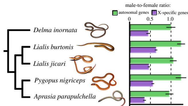
Figure 1. Average relative gene dose ratios between sexes for autosomal genes and X-specific genes of Lialis burtonis examined across five species of pygopodid lizards. The value 1.0 is expected for autosomal or pseudoautosomal genes, whereas 0.5 is consistent with X-specificity. Standard errors are indicated by black bars. (Online version in colour.)
